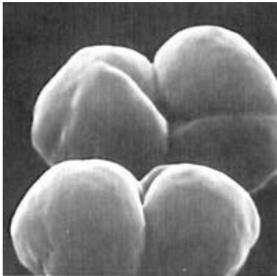
Methanosarcina barkeri
